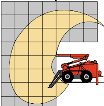
Horizontal drilling, sideways
